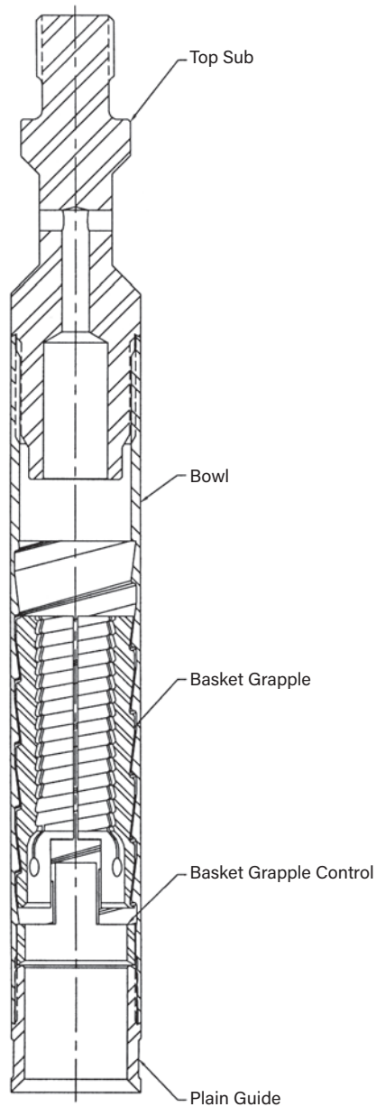
Basket Grapple Assembly
