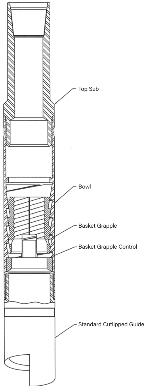
Basket Grapple with Basket Grapple Control
