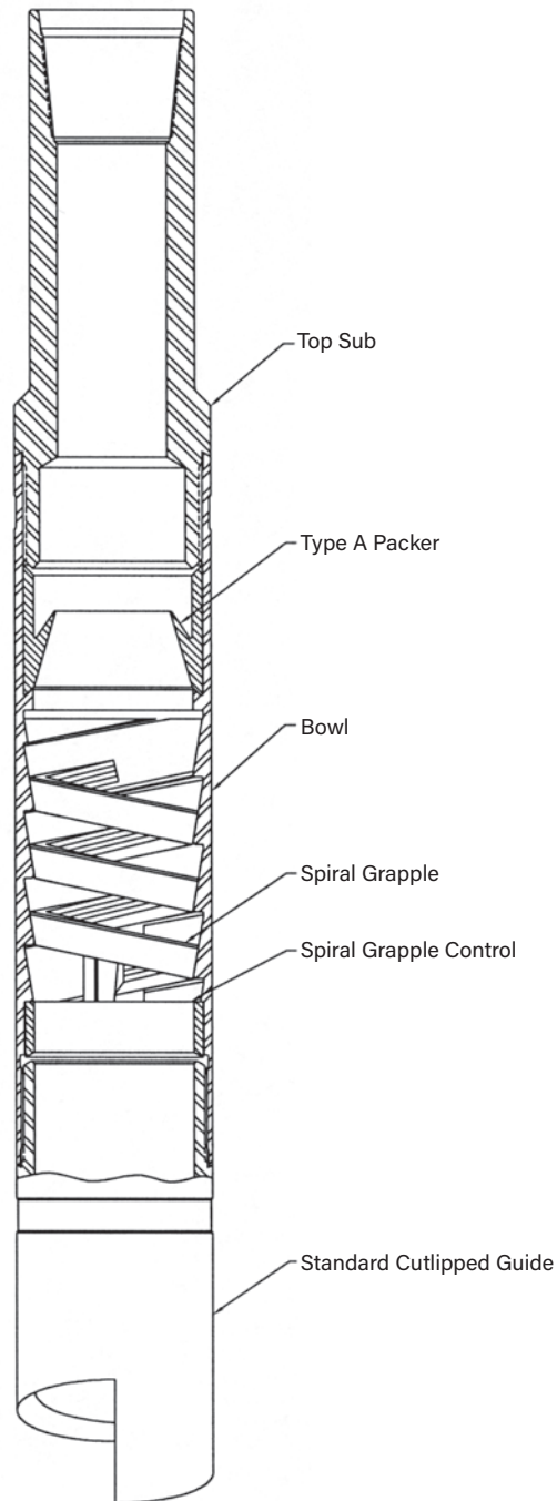
Spiral Grapple with Spiral Grapple Control and Type A Packer
