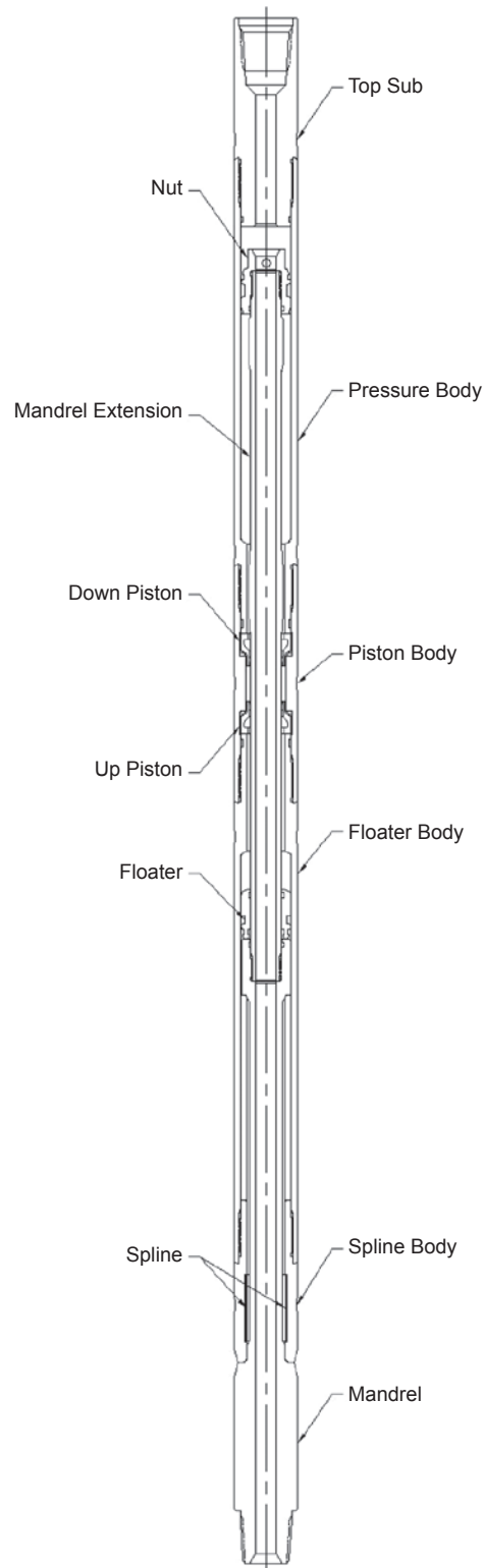
Bi-Directional Coiled Tubing Jar Components
