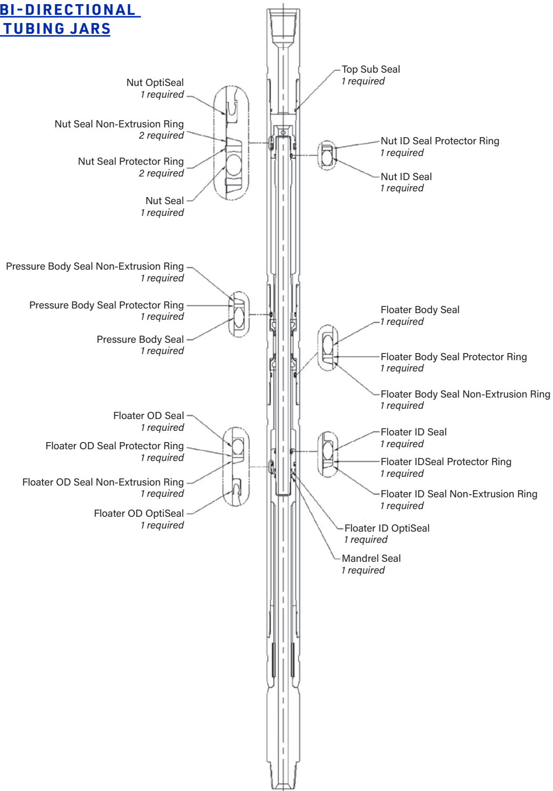
Bi-Directional Coiled Tubing Jar Seal Components
