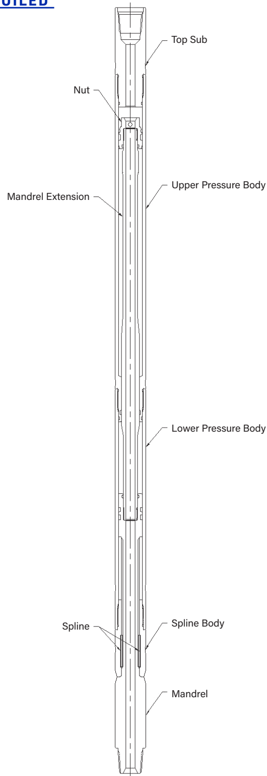
Bi-Directional Coiled Tubing Energizer Components
