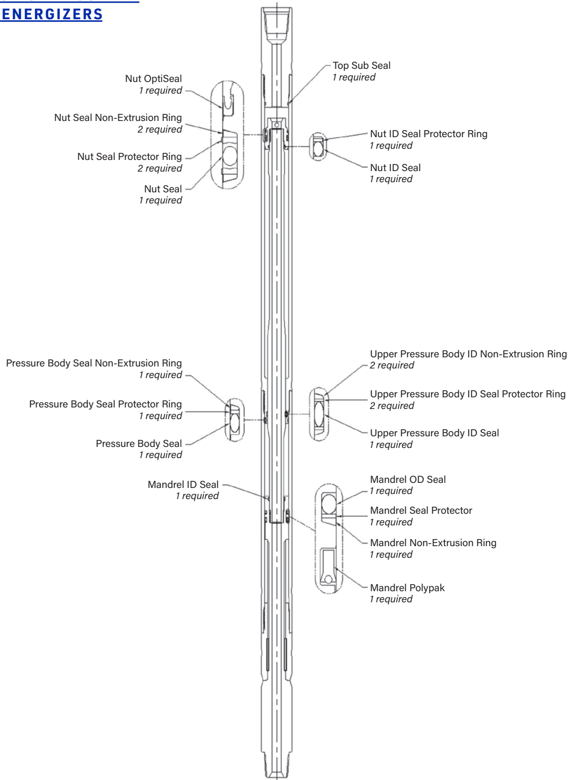
Bi-Directional Coiled Tubing Energizer Seal Components
