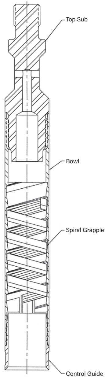
Spiral Grapple Assembly
