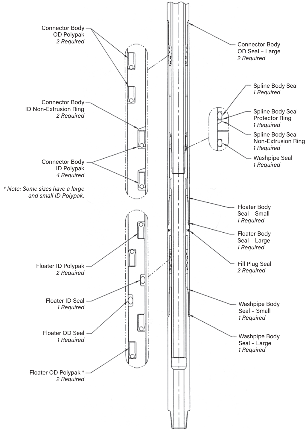
Polypaks and Seals (Lower Half)
